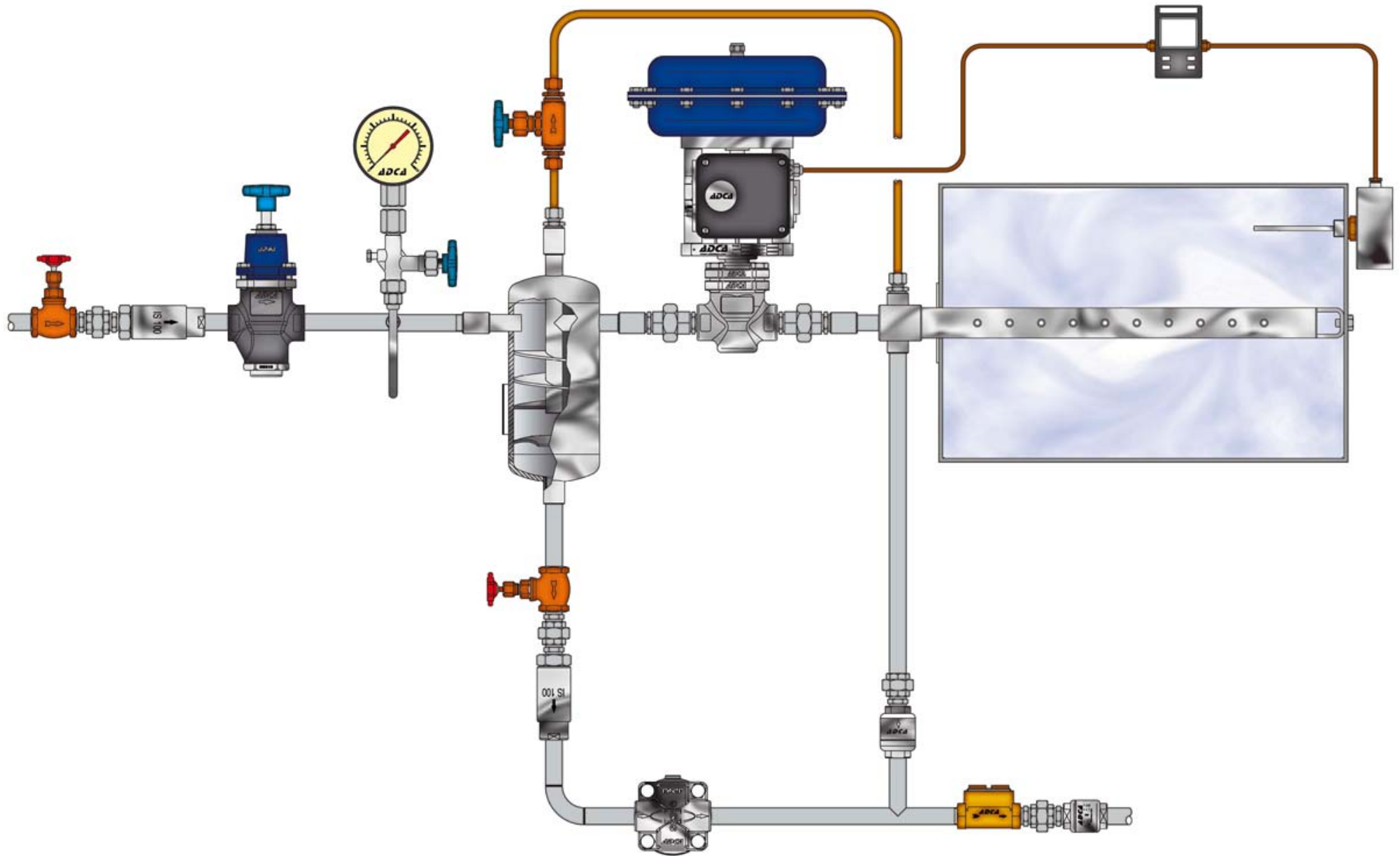
DSH - Direct steam injection humidifiers
